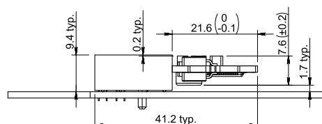
Overall dimensions for horizontal mounting
